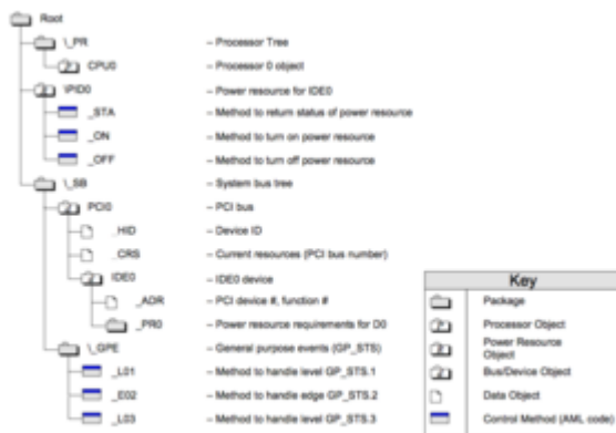
Figure 5-32 Example ACPI Namespace
