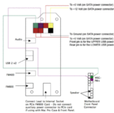
Mosier's revised Hack Pro front panel wiring diagram
