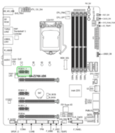
GA-Z270X-UD5 Motherboard Layout
