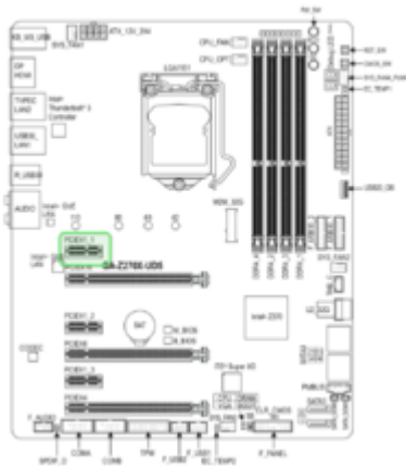
GA-Z270X-UD5 Motherboard Layout
