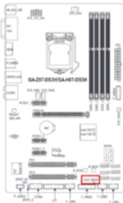
GA-Z87-D53H/GA-H87-D53H Motherboard Layout
