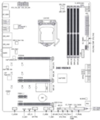
Z490 VISION D Motherboard Layout
