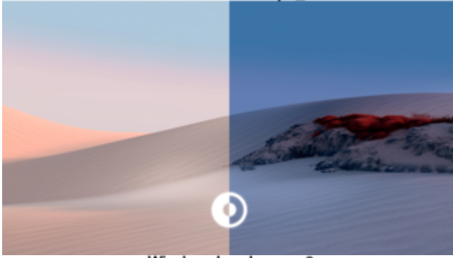
WindowsLandscape_2
